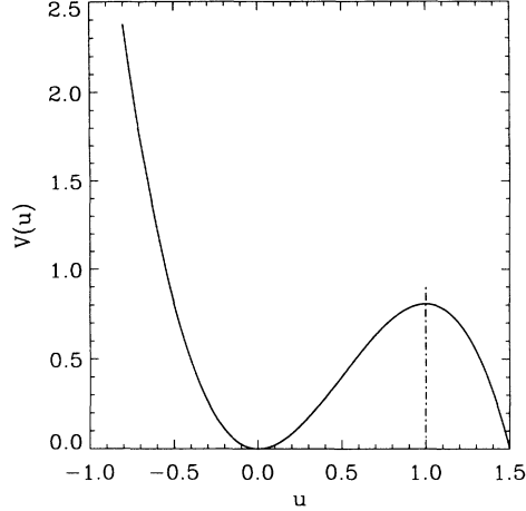
FIG. 1. The on-site potential of the model. We consider only displacements u < 1 .
